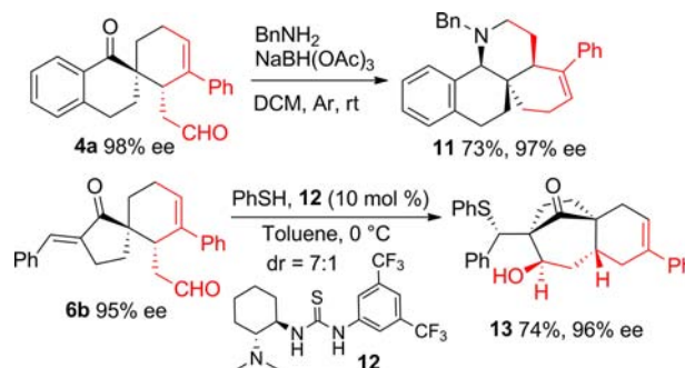
Scheme 5. Transformations of Spirocyclic Products
