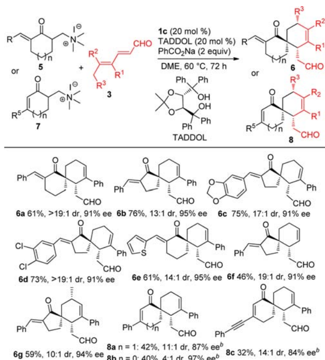
Scheme 3. Substrate Scope of Diels–Alder Reactions with Methiodide Salts from Functional Cyclic Enones a
