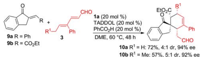
Scheme 4. Synthesis of Highly Substituted Spirocycles
